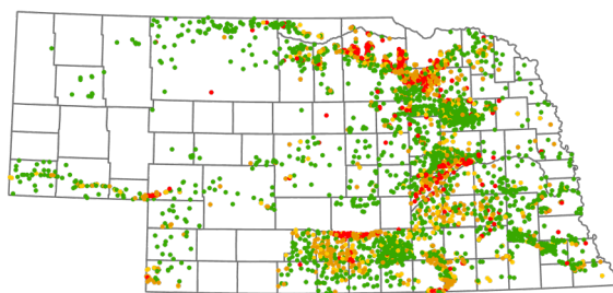
2016 (4275 wells, 4846 analyses)
