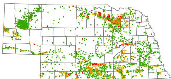
2009 (3428 wells, 4051 analyses)
