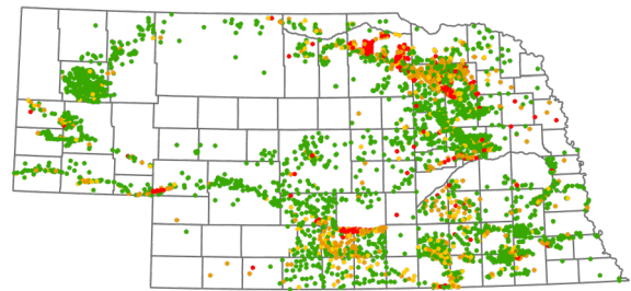
2003 (4422 wells, 5190 analyses)
