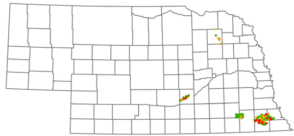
1981 (143 wells, 197 analyses)
