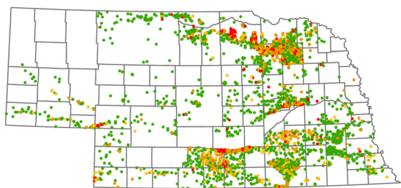
2015 (4252 wells, 4576 analyses)
