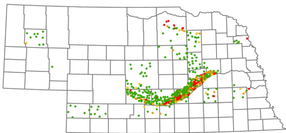
1984 (691 wells, 695 analyses)
