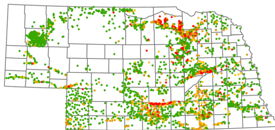
2018 (4317 wells, 4761 analyses)
