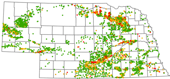
2002 (4321 wells, 5249 analyses)
