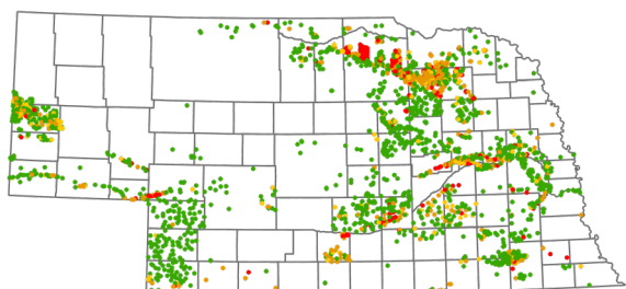
1999 (2883 wells, 3565 analyses)
