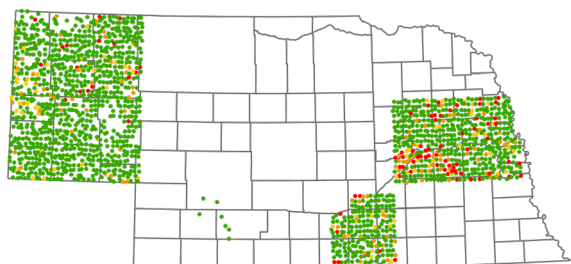
1979 (1843 wells, 1844 analyses)
