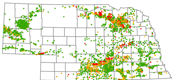
2005 (4275 wells, 5284 analyses)
