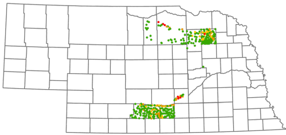
1980 (402 wells, 469 analyses)
