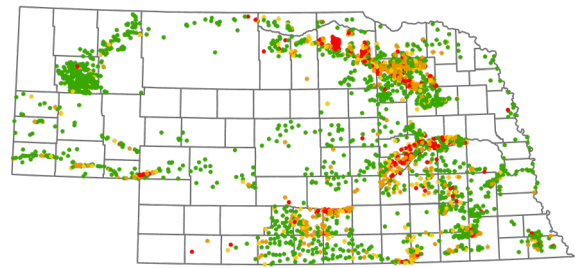
2001 (3243 wells, 3866 analyses)
