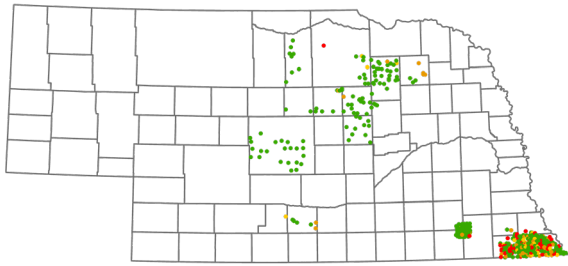
1982 (506 wells, 519 analyses)
