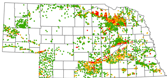
2017 (4641 wells, 49013 analyses)
