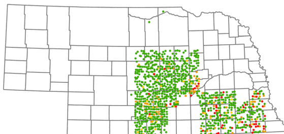
1978 (1056 wells, 1081 analyses)
