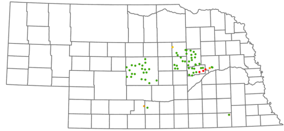
1983 (65 wells, 67 analyses)
