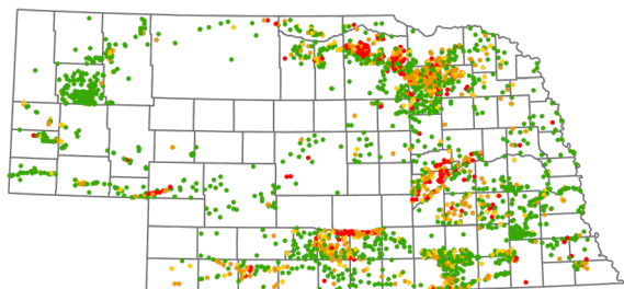
2007 (3099 wells, 3610 analyses)
