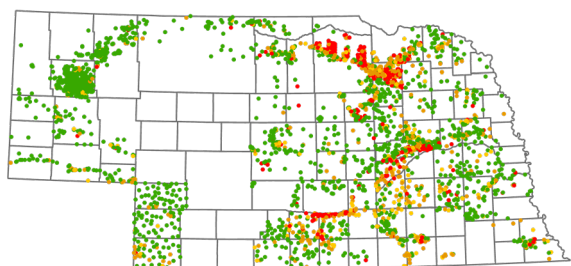
2019 (3797 wells, 3931 analyses)
