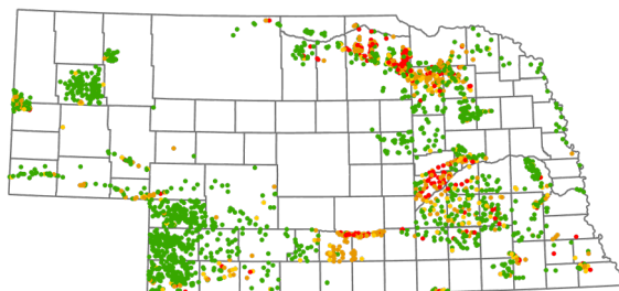
1998 (2424 wells, 3156 analyses)
