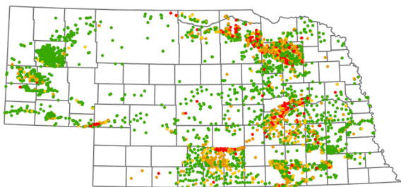
2004 (3977 wells, 4944 analyses)
