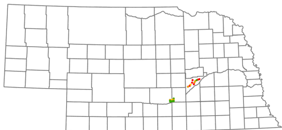
1977 (45 wells, 45 analyses)
