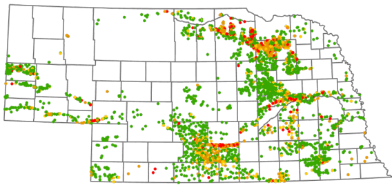
2000 (3502 wells, 4473 analyses)
