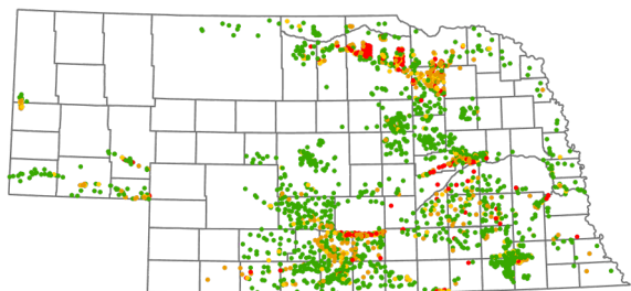
1997 (2623 wells, 3604 analyses)
