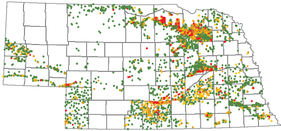
2017 (4245 wells, 4482 analyses)
