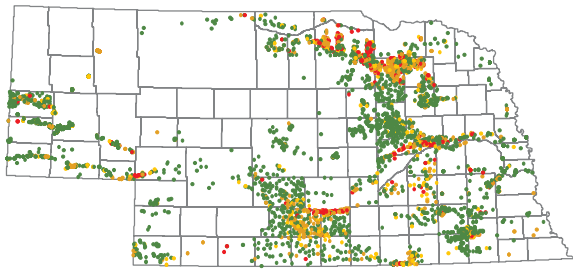
2000 (3503 wells, 4477 analyses)
