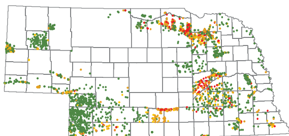
1998 (2425 wells, 3157 analyses)
