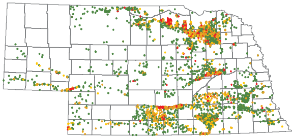
2015 (4254 wells, 4579 analyses)
