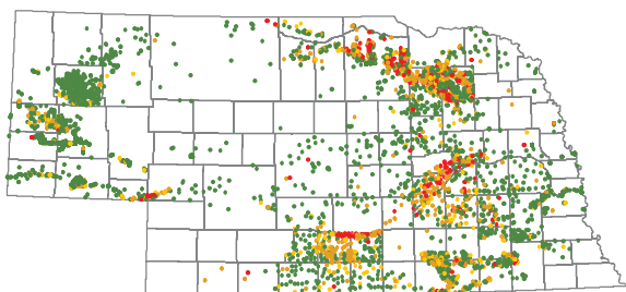
2004 (3978 wells, 4945 analyses)
