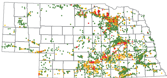
2014 (4344 wells, 4804 analyses)
