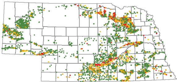
2002 (4323 wells, 5251 analyses)
