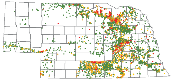
2016 (4278 wells, 4849 analyses)
