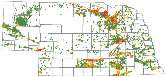
2012 (4742 wells, 5438 analyses)
