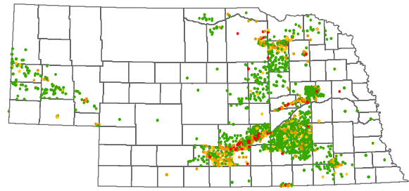
1991 (1918 wells, 2871 analyses)
